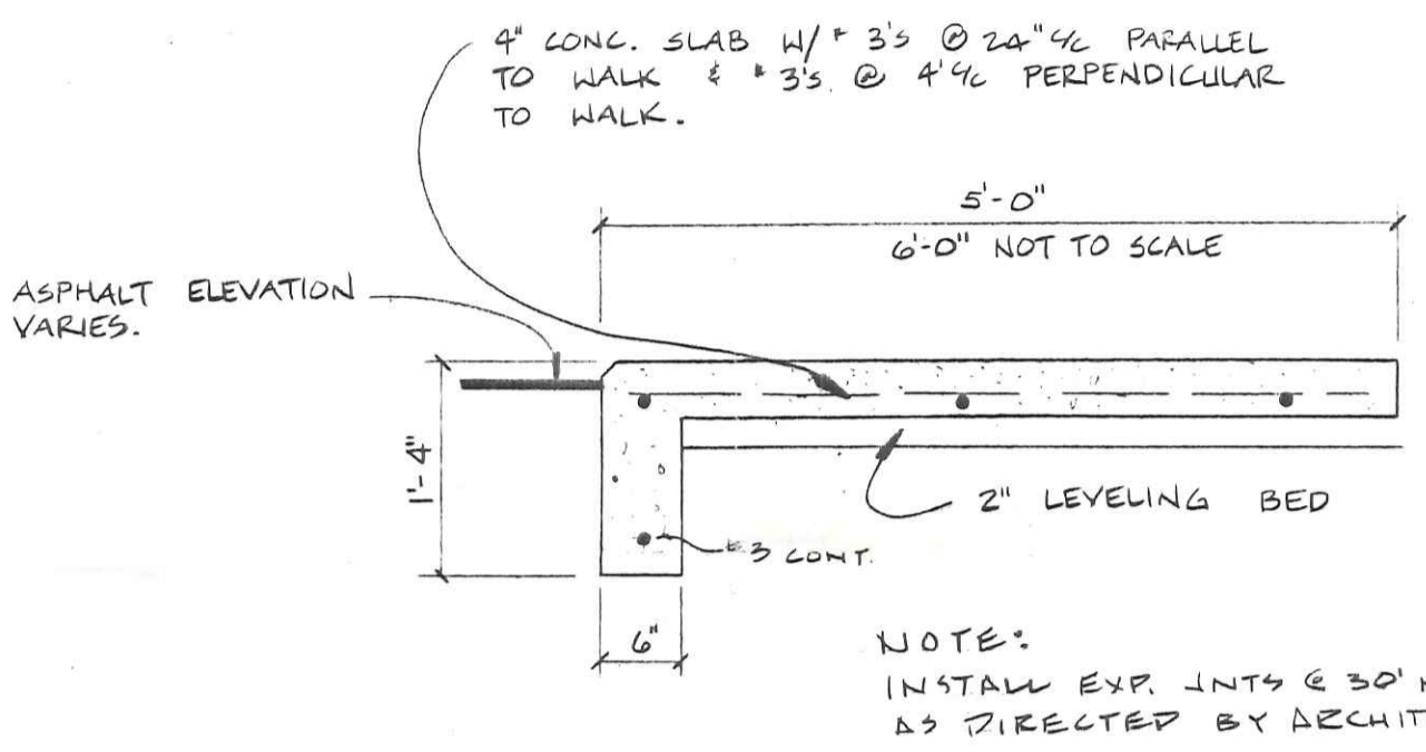
WALK DETAIL SCALE: 3/4" = 1'-0"
